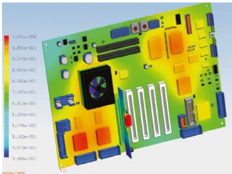
Simulation capabilities include thermal and flow analysis.
